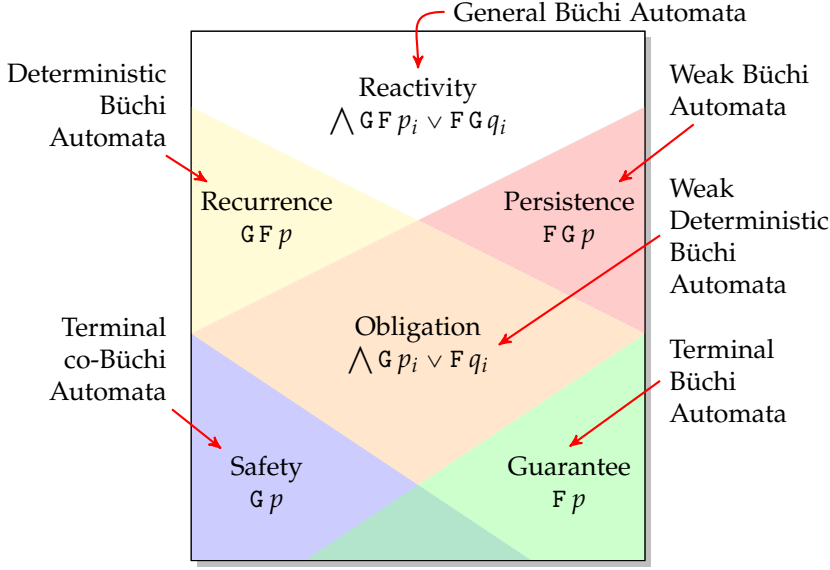
Figure 4.1.: The temporal hierarchy of Manna and Pnueli [13] with their associated classes of automata [5]. The formulas associated to each class are more than canonical examples: they show the normal forms under which any LTL formula of the class can be rewritten, assuming that p, p_i, q, q_i denote subformulas involving only Boolean operators, X , and past temporal operators (Spot does not support the latter).
