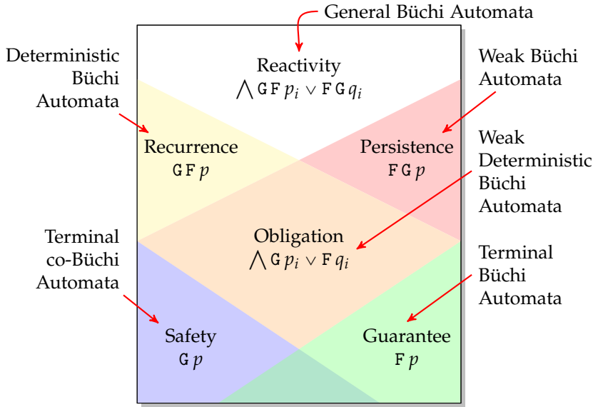
Figure 4.1.: The temporal hierarchy of Manna and Pnueli [14] with their associated classes of automata [5]. The formulas associated to each class are more than canonical examples: they show the normal forms under which any LTL formula of the class can be rewritten, assuming that p, p_i, q, q_i denote subformulas involving only Boolean operators, X , and past temporal operators (Spot does not support the latter).
